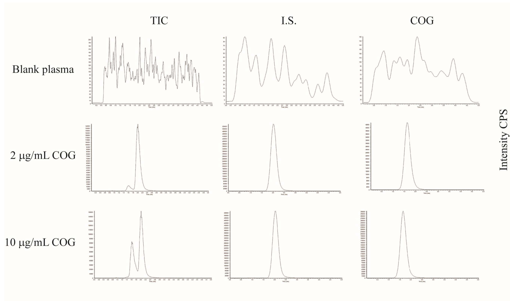
Fig. S1: The chromatograms of COG and the internal standard from COG stability-test mouse plasma samples. The total ion current (TIC) chromatogram and extracted ion chromatograms of mouse plasma spiked with 1000 ng/mL I.S. and 2 µg/mL or 10 µg/mL COG are presented.
