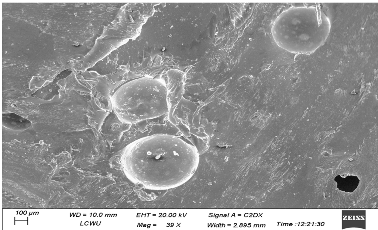
Supplementary fig. 2: SEM analysis of OM-co-poly(AA) hydrogel
