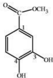
Methyl protocatechuate (1)
