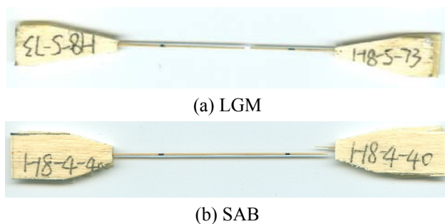
Fig. 7: Tensile test failure code
