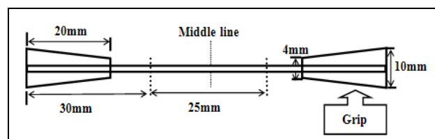
Fig. 4: Vascular Bundle Sample for Tensile Test.
