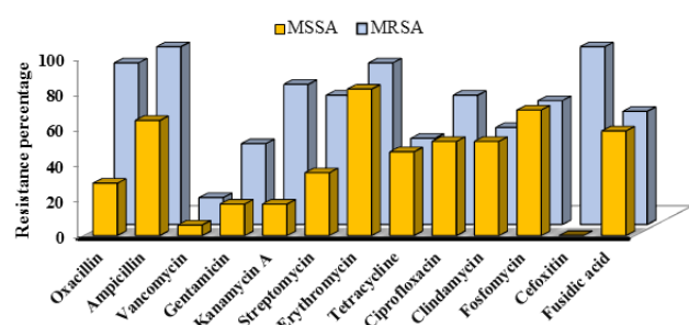
Fig. 4: Comparative illustration of Antibiotic resistance between MSSA and MRSA
