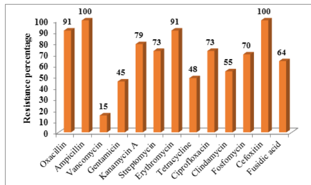
Fig. 3: Antibiotic Resistance Profile of MRSA
