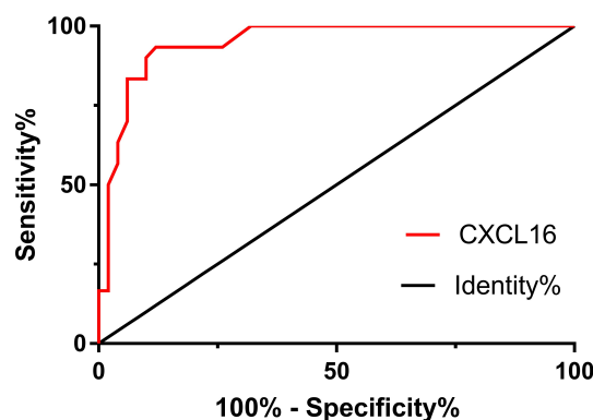
Fig. 3: ROC curve of CXCL16 in the diagnosis of ACS patients.
