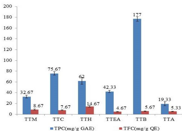
Fig. 1: TPC and TFC of TTM extract and its fractions
