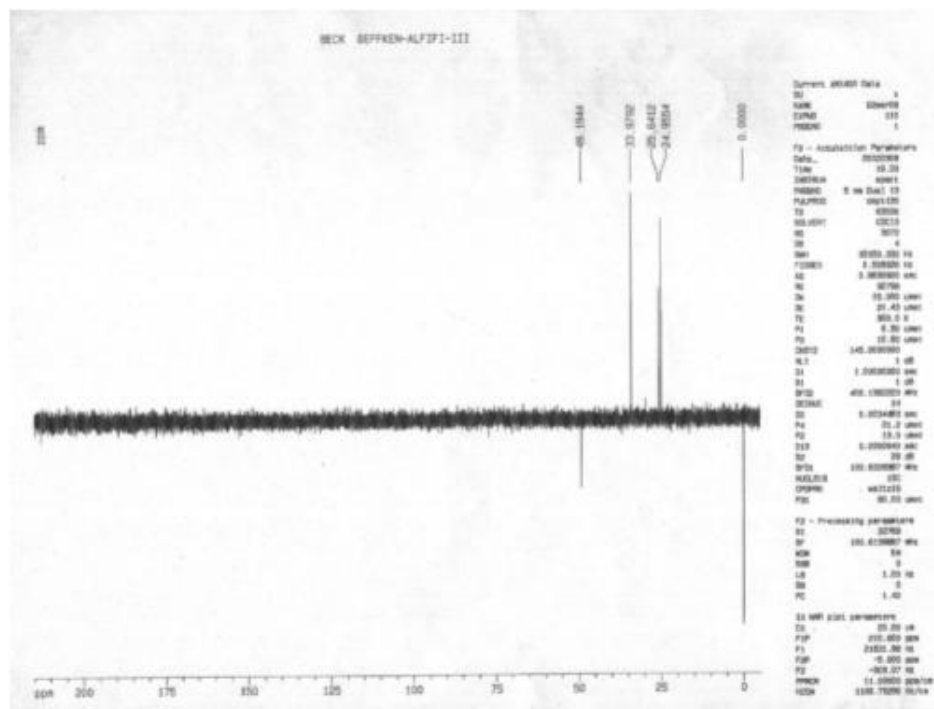
Fig. 1: 13 C-NMR of N,N'- dicyclohexylurea with DEPT (135)
