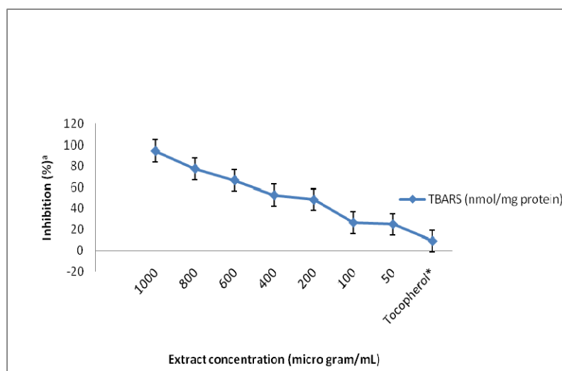
Fig. 2: Effect of chloroform root extract of DG on ferrous sulphate induced lipid peroxidation in rat liver homogenate.
